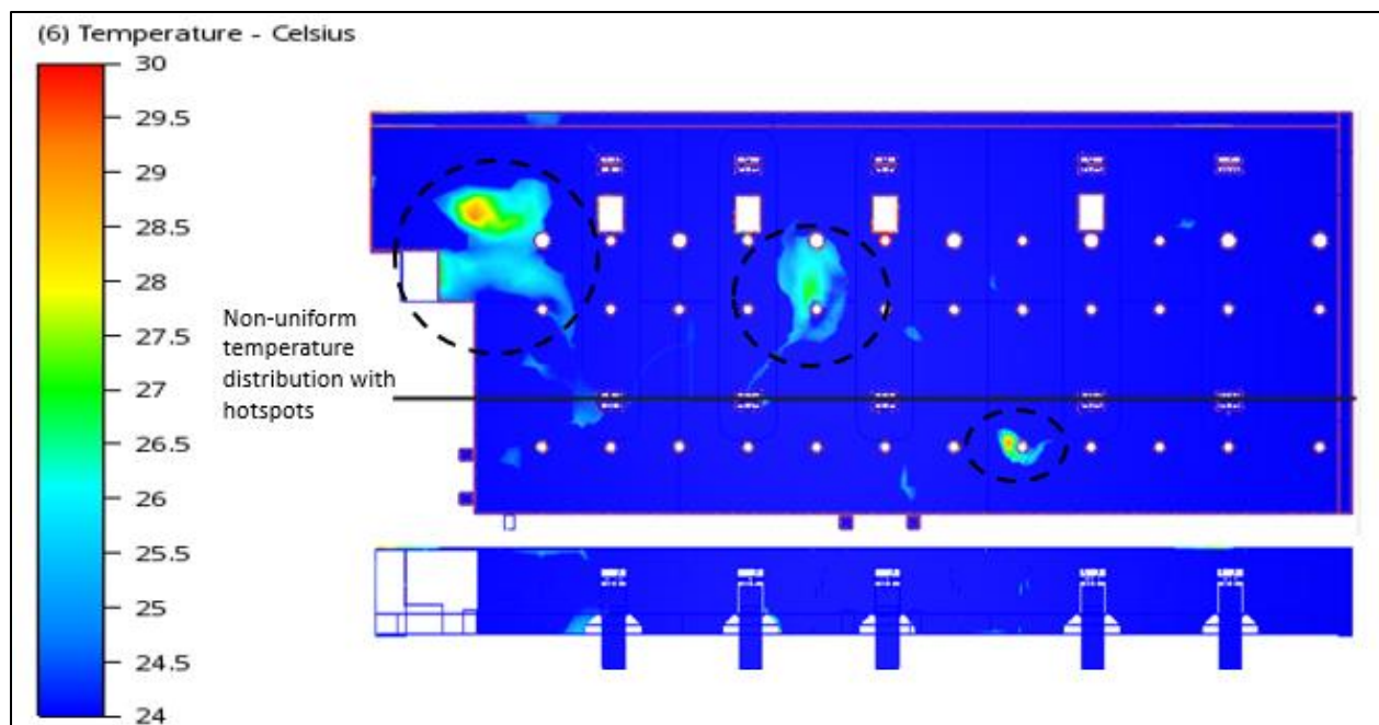
Temperature distribution
