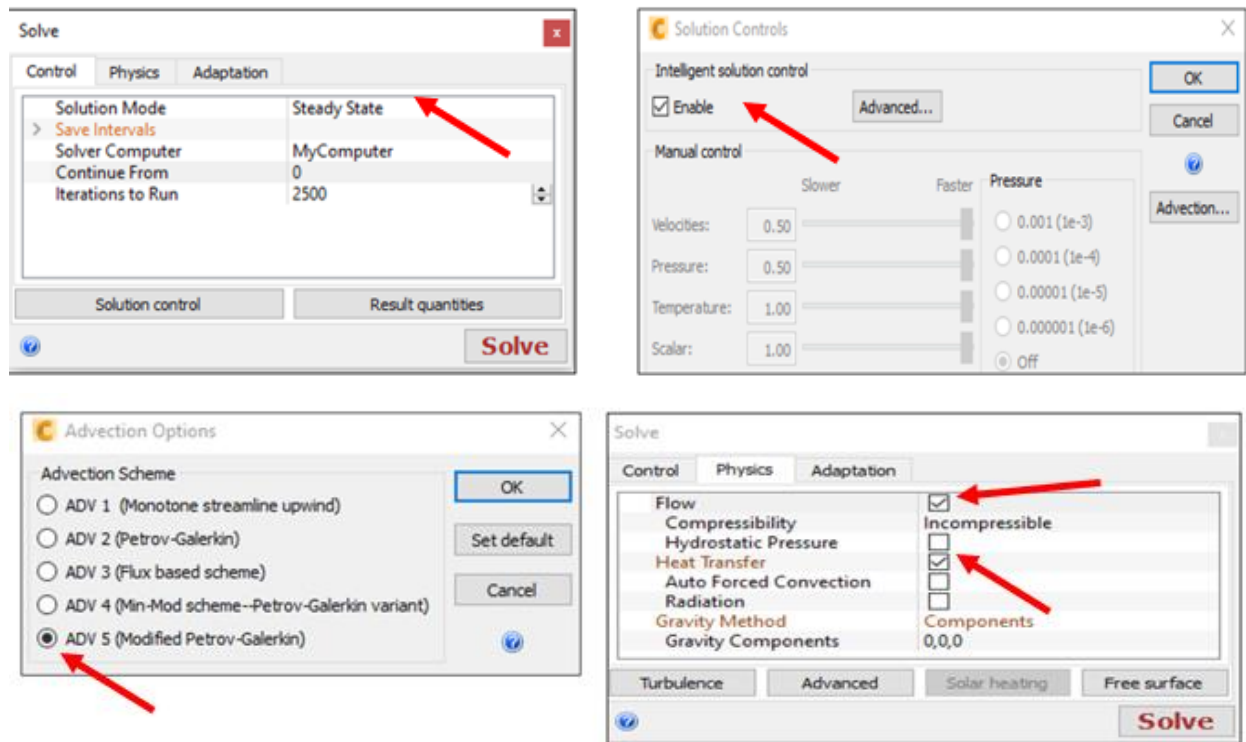
Solver settings for flow analysis (Intelligent solution control (ISC)-On, Advection Scheme 5)
