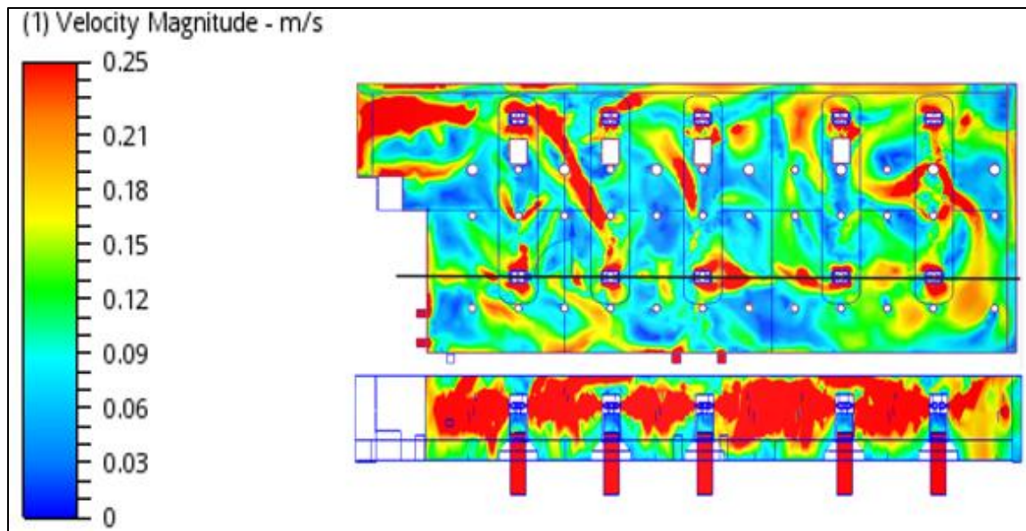
Velocity distribution
