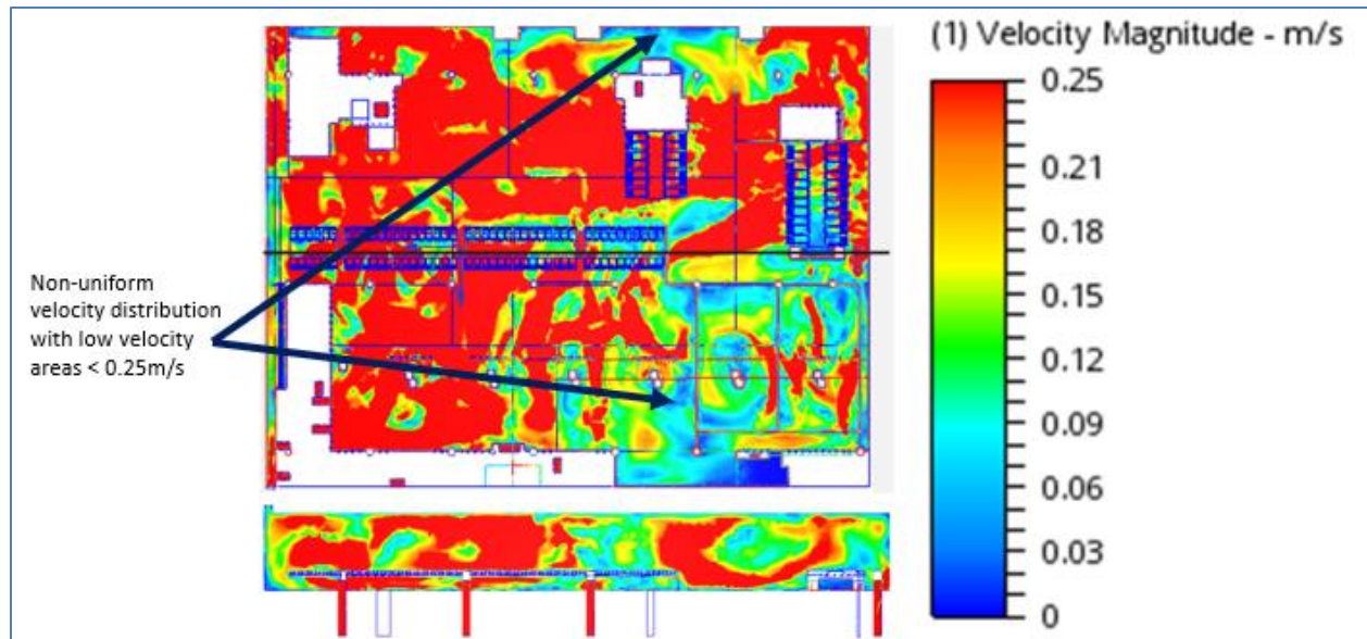
Velocity distribution
