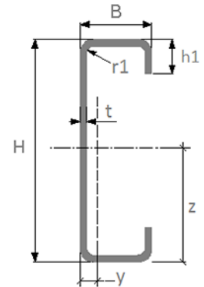
C Profile with Lips
