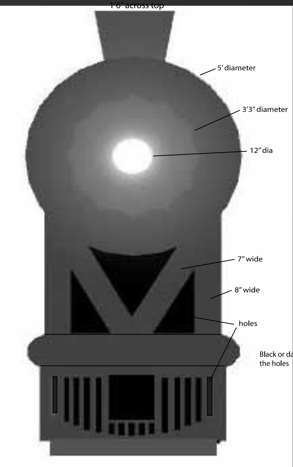
Train Front On the Twentieth Century Schweppe Jan 2008 approx 3/4\" = 1'
