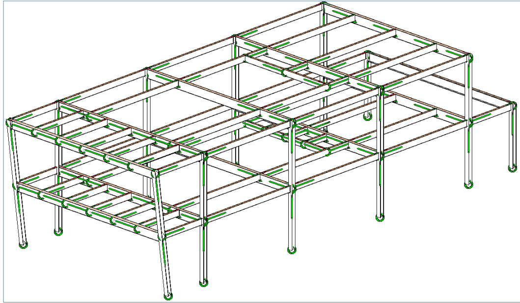
FIGURE 36: CONNECTION ELEMENTS DISPLAYED AS SYMBOLS
