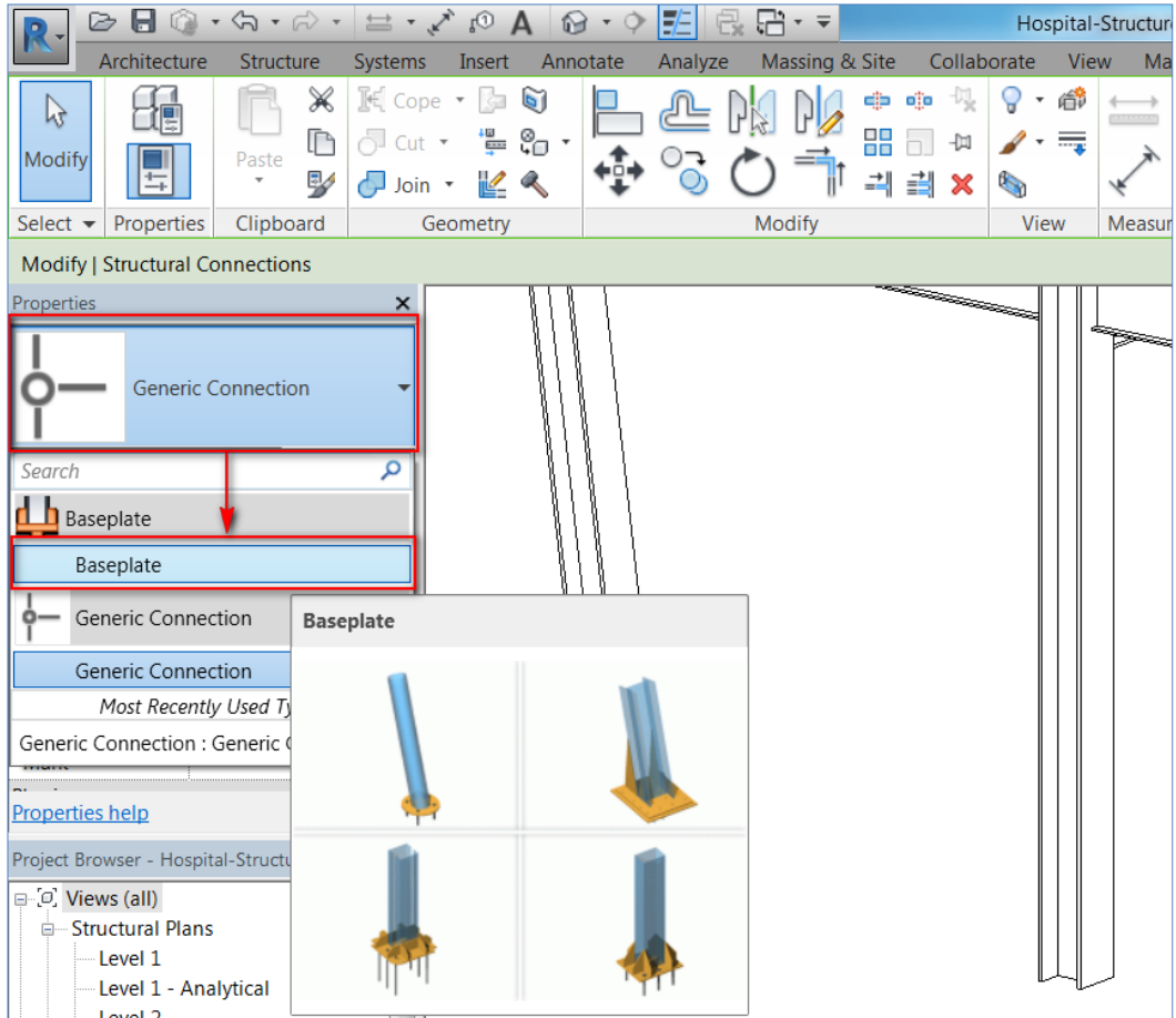
FIGURE 34: SELECTING THE BASE PLATE CONNECTION FOR THE COLUMN
