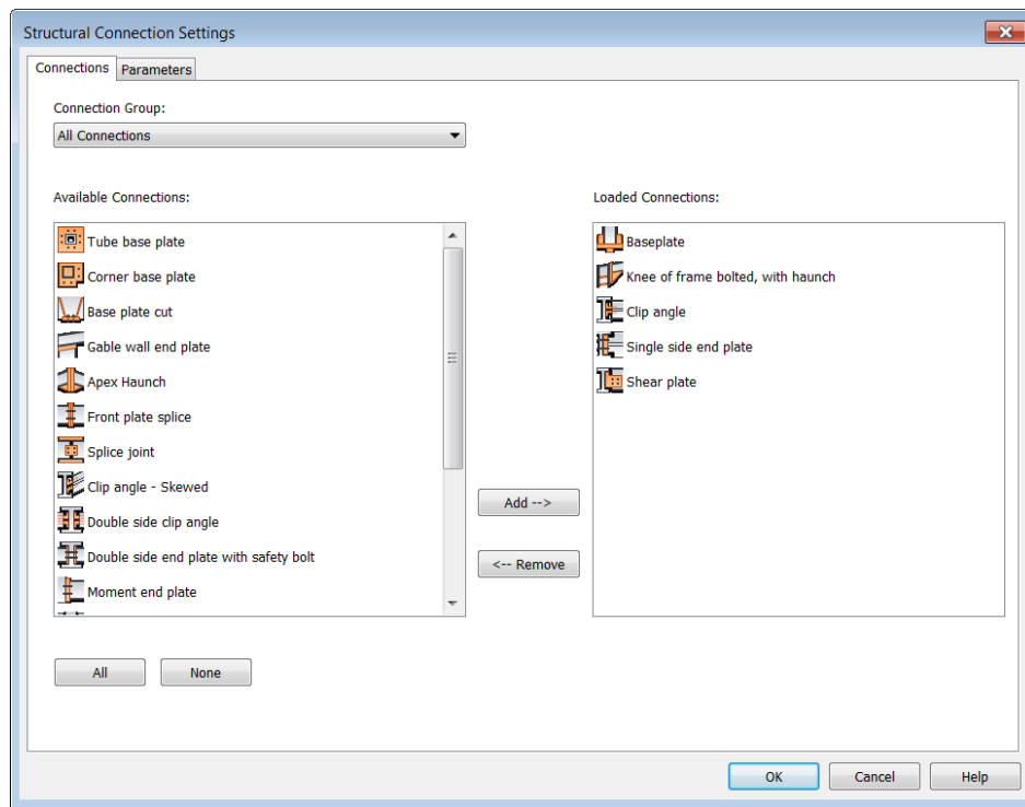
FIGURE 32: THE CONNECTION LOADED FOR USE
