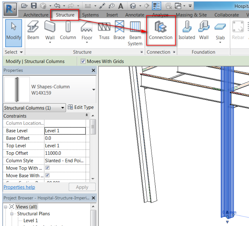
FIGURE 33: SELECTING THE COLUMN TO INSERT THE BASE PLATE CONNECTION
